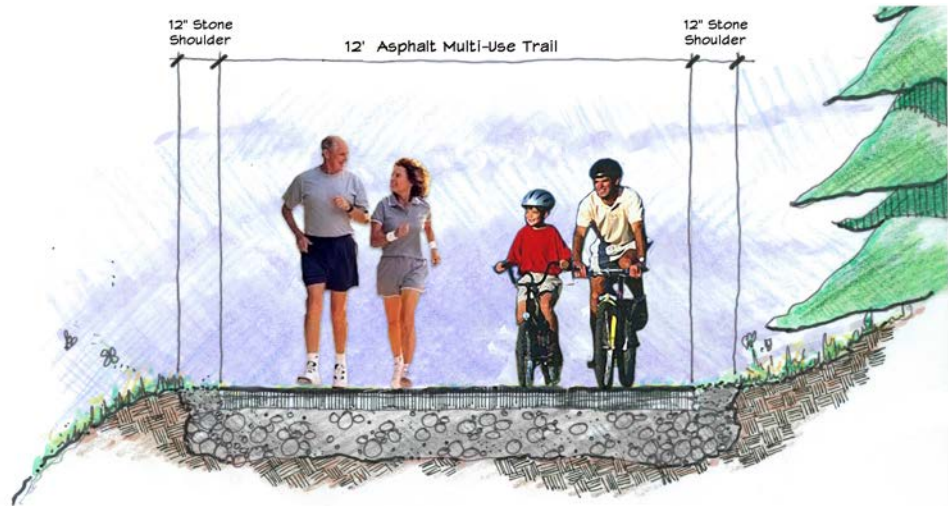
TYPICAL 12' MULTI-USE TRAIL SECTION THROUGH PARK WITH SHOULDERS N.T.S.
